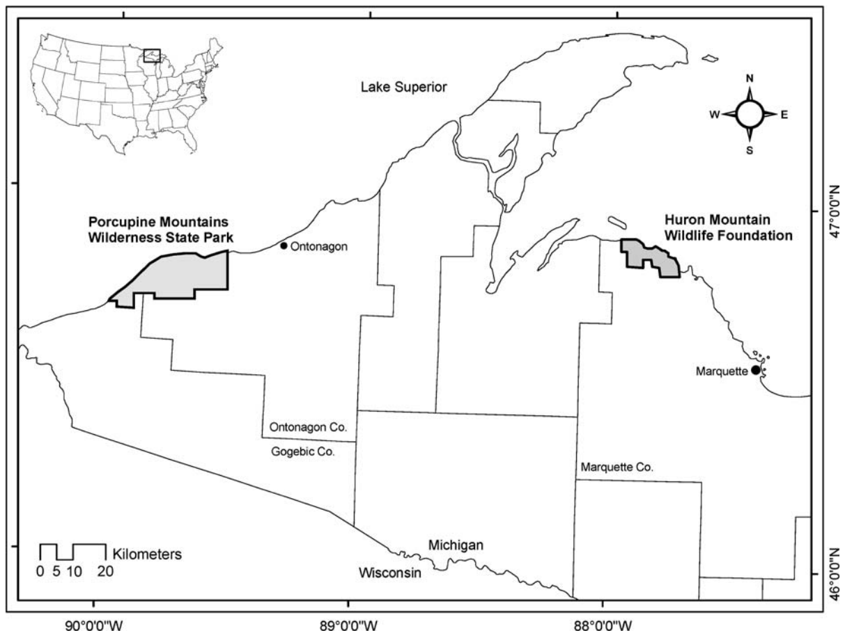
Fig. 1 Location of the study areas in the Huron Mountain Reserve Area (HMRA) and Porcupine Mountain Wilderness State Park (PMWSP), upper MI, USA
