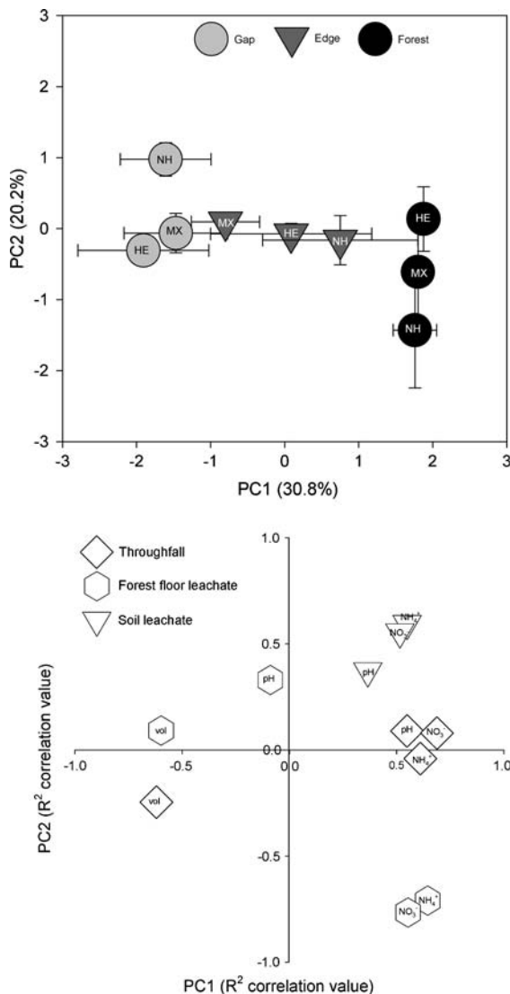
Fig. 4 Principal components and loadings for forest water transfers in gap, edge, and forest plots throughout the 2006 growing season in late-successional northern hardwood–hemlock forests of the upper Great Lakes region, USA. Principal component analyses were performed on 2006 growing season means. N = 27
