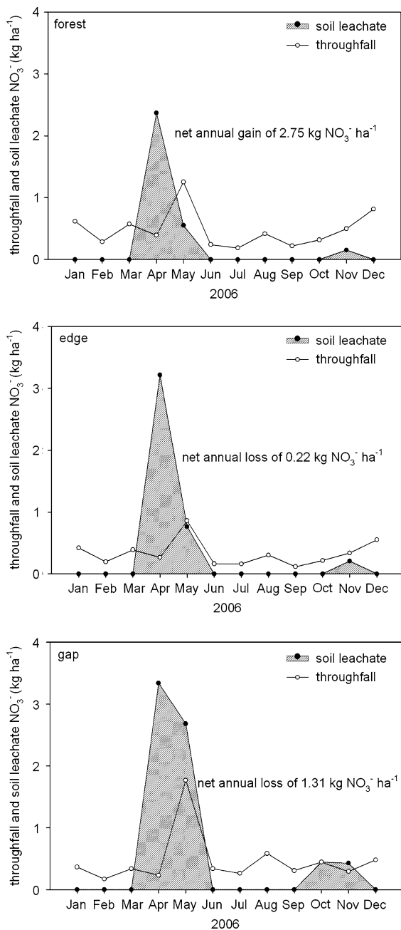
Fig. 5 Nitrate inputs in throughfall and outputs in soil leachates in gap, edge, and forest plots throughout 2006 in late-successional northern hardwood–hemlock forests of the upper Great Lakes region, USA. Values are monthly modeled response using WATBAL
