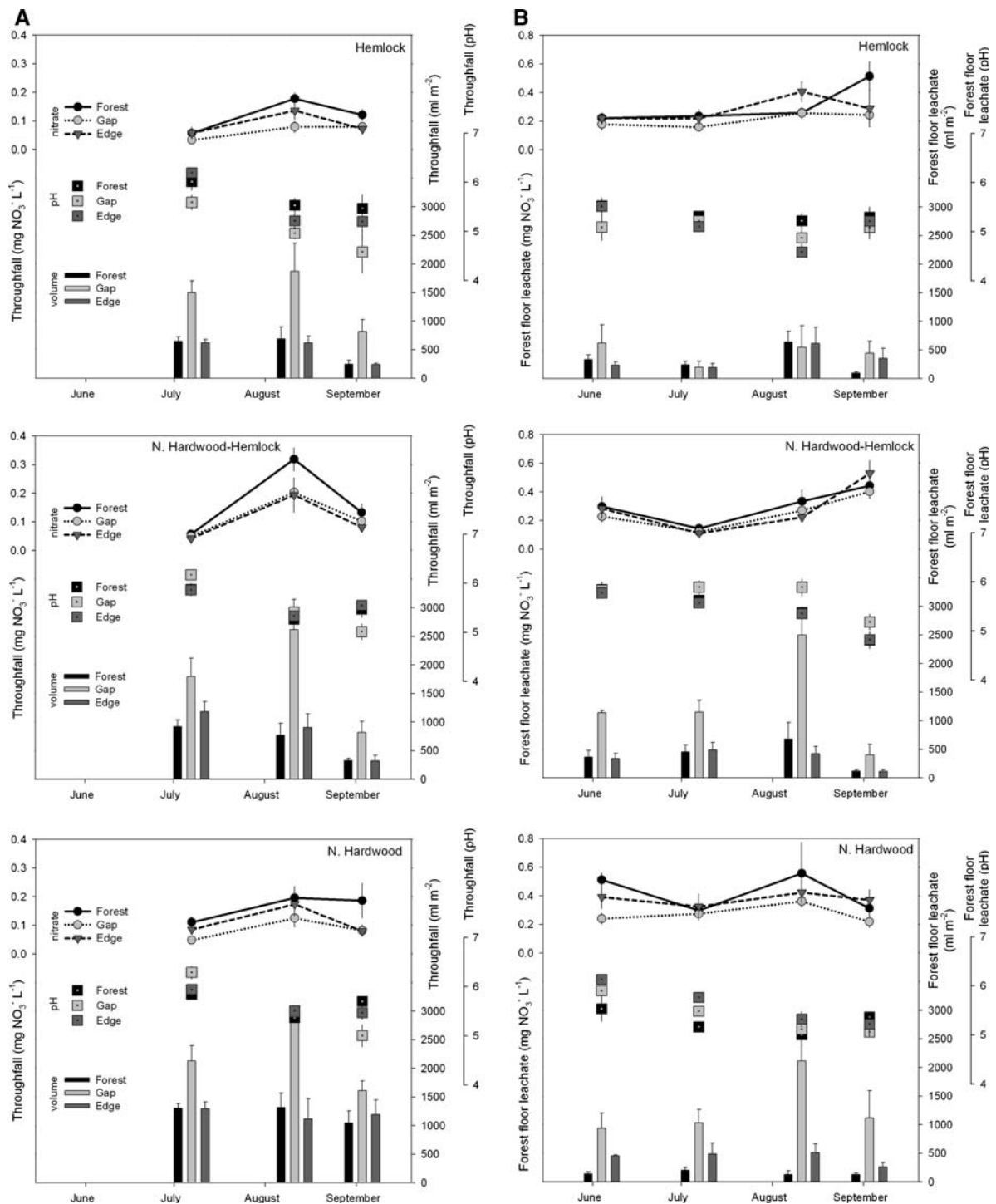
Fig. 3 Flux volume, pH, and nitrate in (a) throughfall, (b) forest floor leachate, and (c) soil leachate in gap, edge, and forest plots throughout the 2006 growing season in late-successional hemlock, northern hardwood–hemlock, and northern hardwood forests of the upper Great Lakes region, USA. Treatments (gap, edge, and forest), cover types (northern
