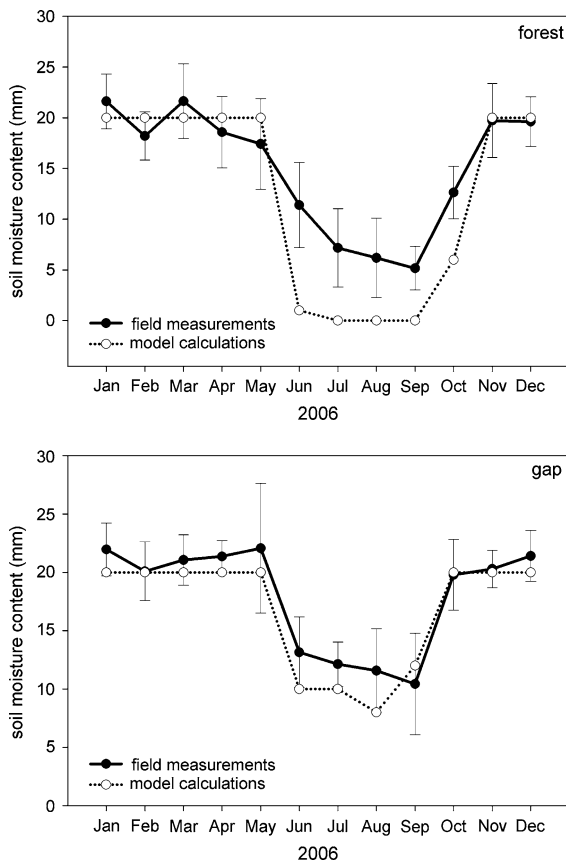
Fig. 2 Soil moisture contents in forest and gaps as measured in the field and as estimated for monthly intervals by the WATBAL model. Field measurements calculated from four gaps and four adjacent forest plots (sites H8, H9, P7, and P9, see Table 1). Error bars are the standard error of means. N = 8
